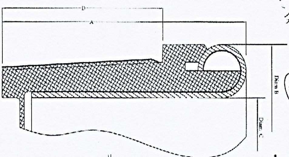
BOX Protector
